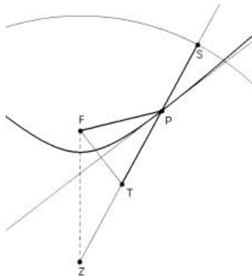
Fig. 45: Computersimulation
