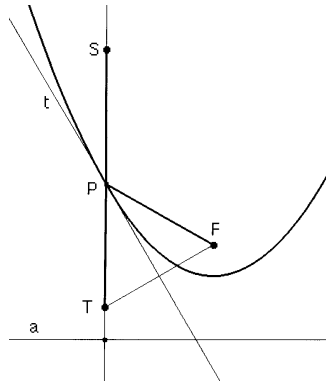
Fig.43: Computersimulation
