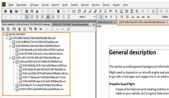
Figure 2: Flache UUID-Hierarchie
