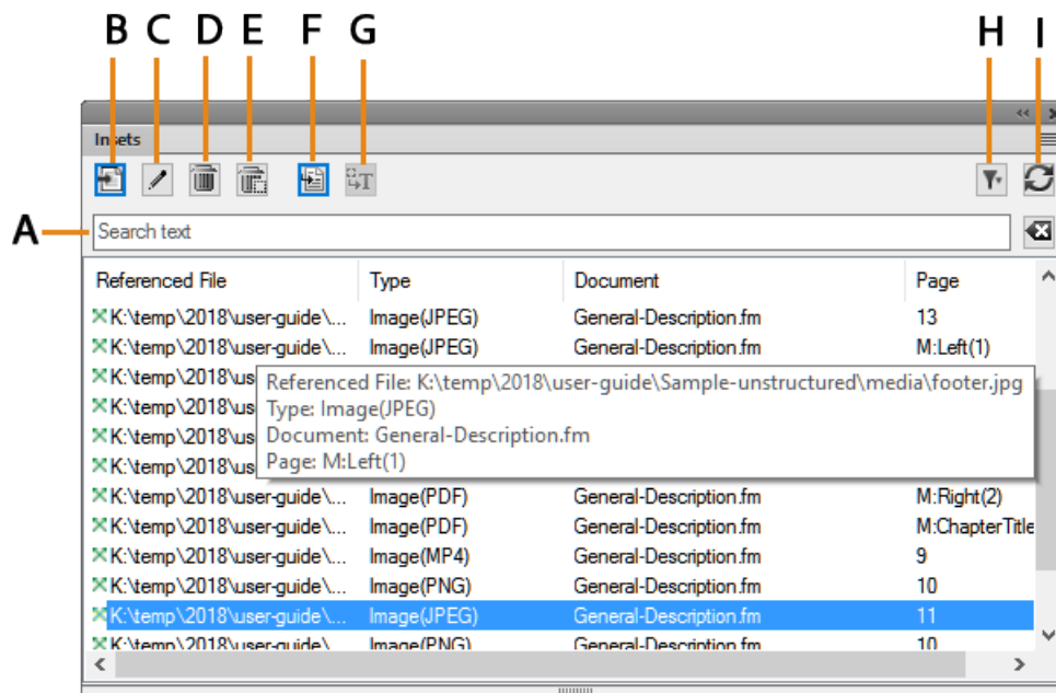
Figure 1: Insets-Bedienfeld
