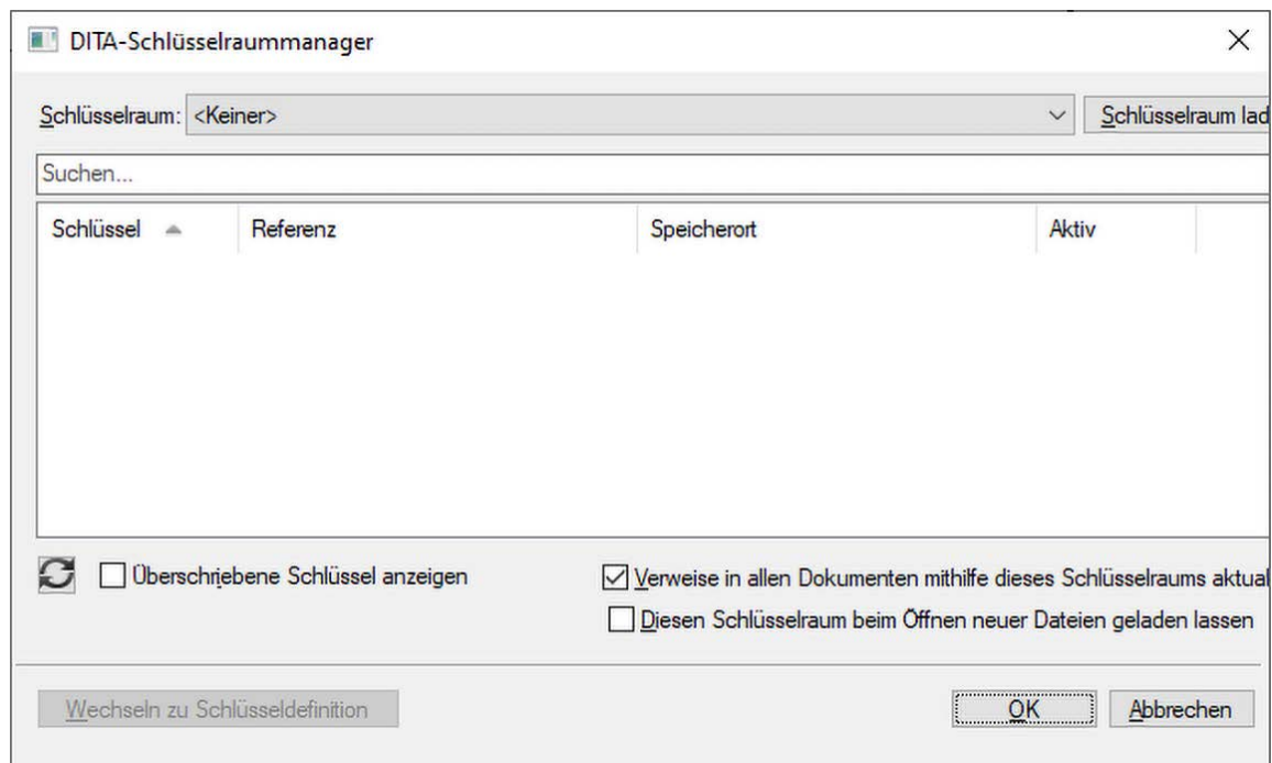
Figure 2: Dialogfeld „DITA-Schlüsselraummanager“
