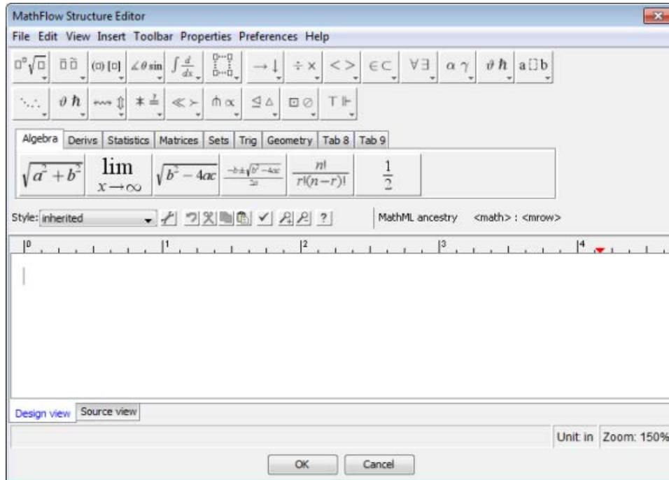
Figure 2: Struktur-Editor
