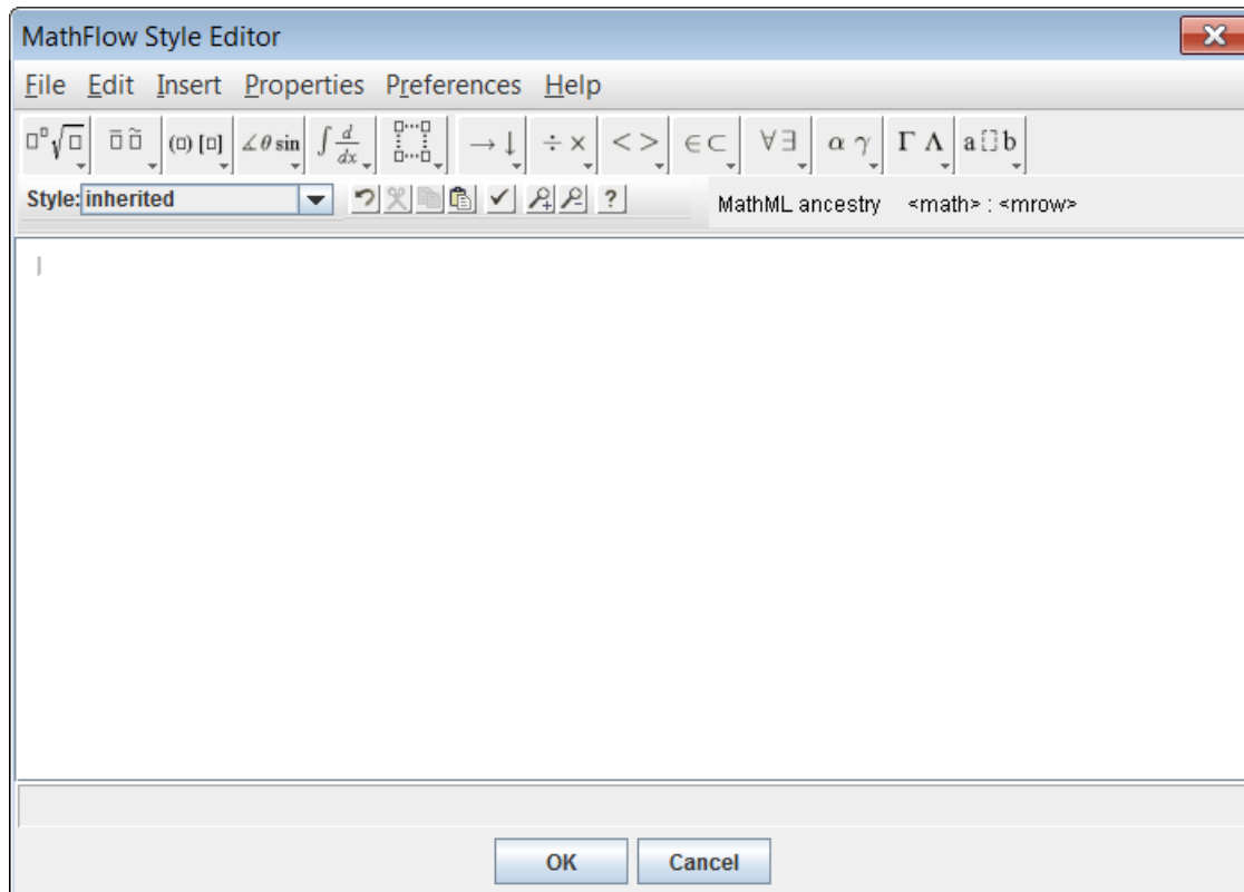
Figure 1: Stil-Editor
